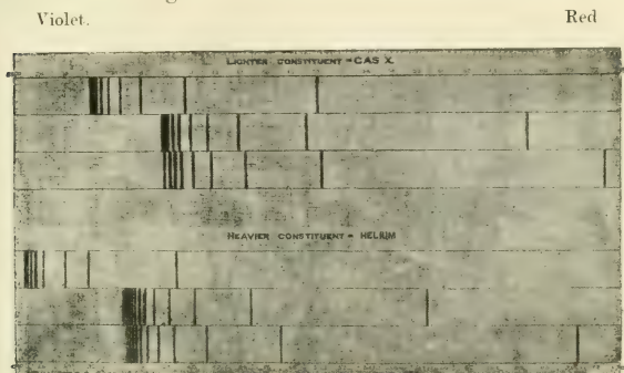
FIG. 11.—The series in the cleveite gases.
